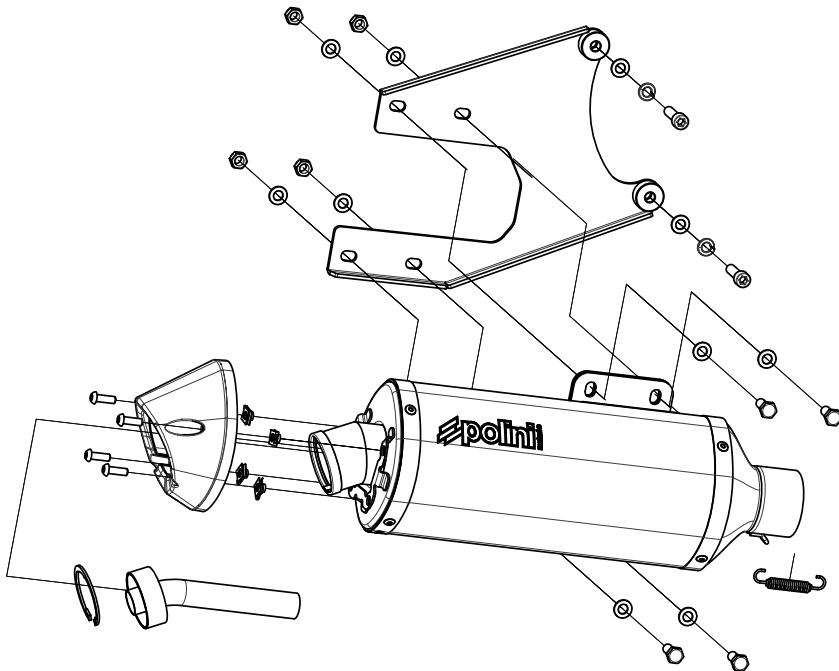
Silencer
